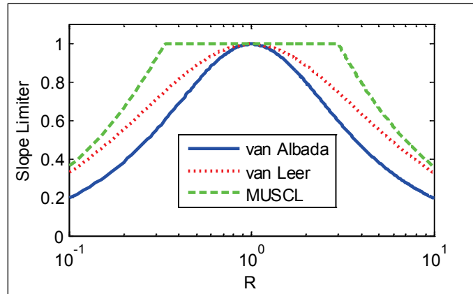
Figure 3-6. Comparison of three different slope limiters.
