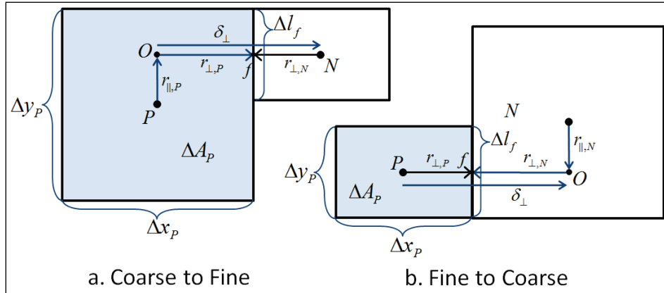
Figure 3-4. Schematic showing interface interpolation: (a) coarse to fine and (b) fine to coarse.
