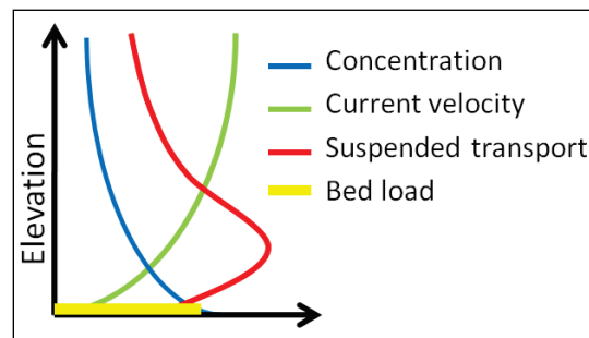
Figure 2-3. Schematic of sediment and current vertical profiles.
