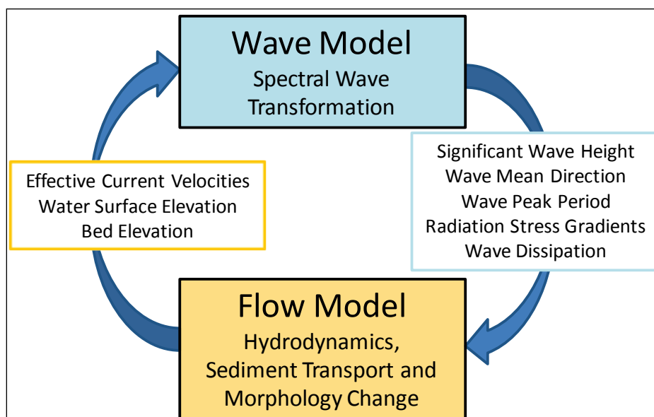
Figure 3-9. Coupling process between CMS-Flow and CMS-Wave.
