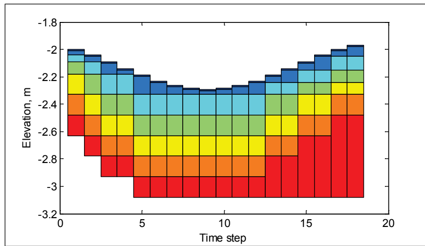
Figure 3-8. Schematic showing an example bed layer evolution. Colors indicate layer number and not bed composition.
