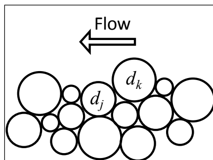
Figure 2-6. Schematic of the exposure height of bed sediment grains.
