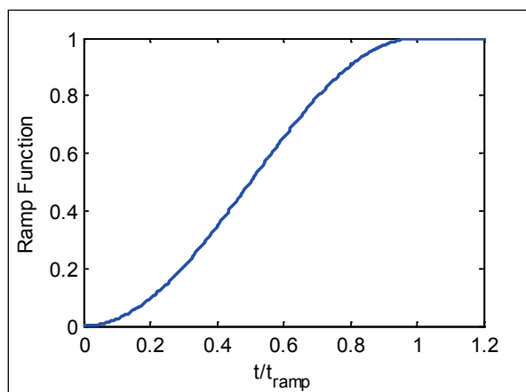
Figure 3-7. Ramp function used in CMS.
