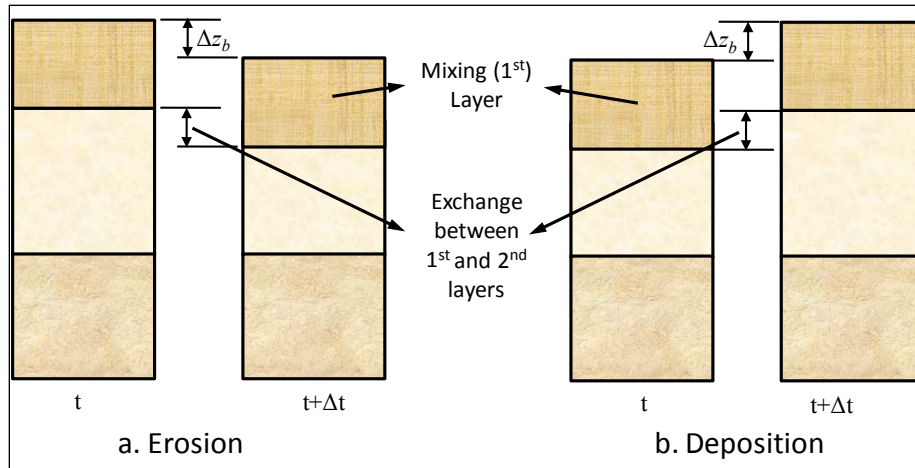
Figure 2-5. Multiple bed layer model of bed material sorting (after Wu 2007).
