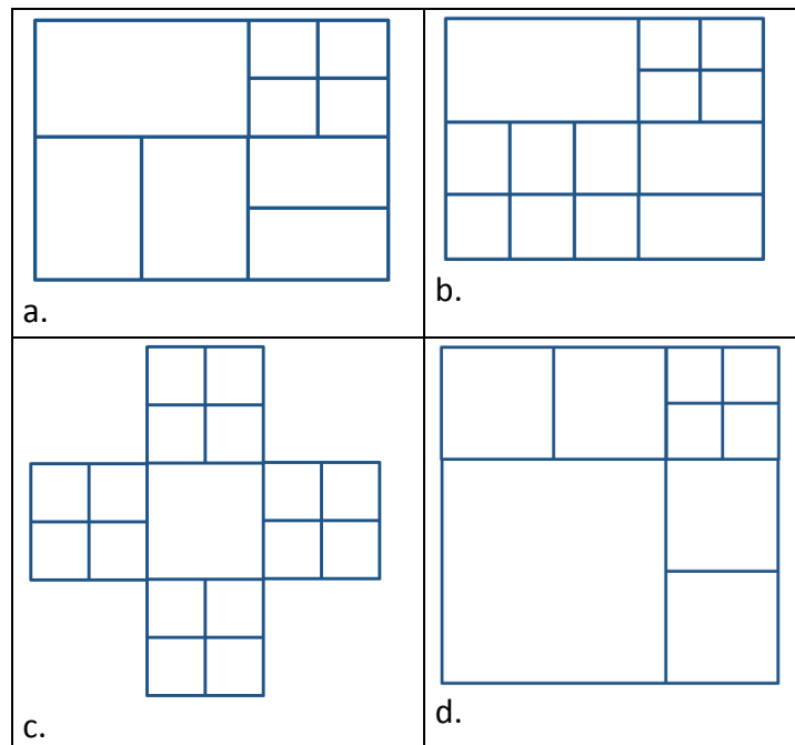
Figure 3-1. Examples of invalid Cartesian computational grids.
