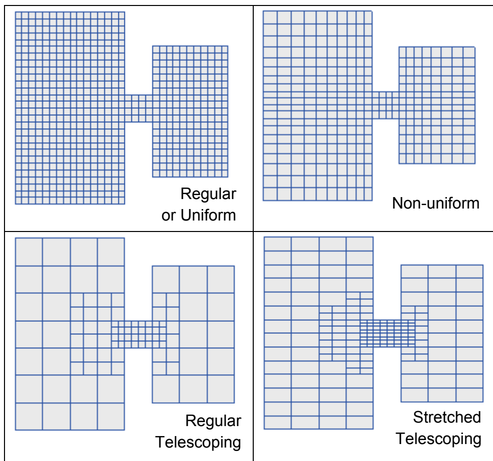
Figure 3-2. Types of Cartesian grids supported by the SMS interface and CMS-Flow.
