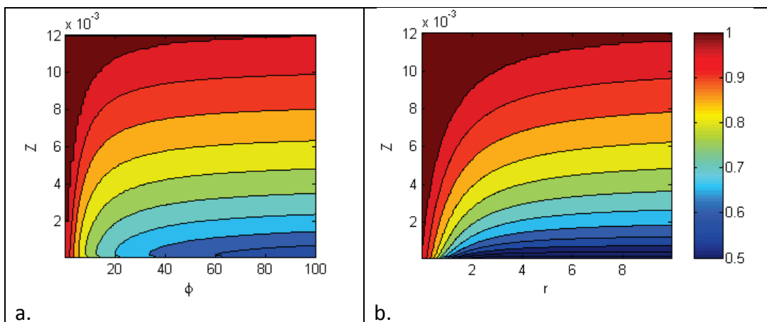
Figure 2-4. Suspended load correction factors based on the logarithmic velocity profile and (a) exponential and (b) Rouse suspended sediment profile. The Rouse number is r = \omega_s / (\kappa u_* ) .
