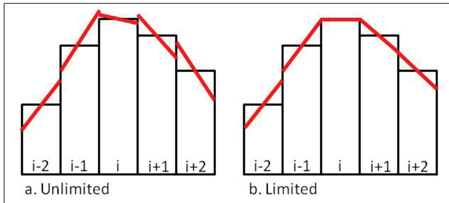
Figure 3-5. Schematics showing examples of (a) non-limited and (b) limited linear reconstructions.
