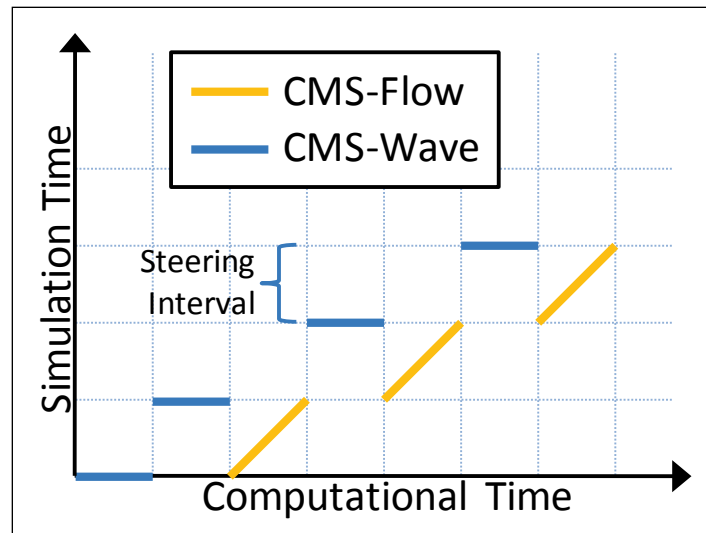
Figure 3-10. Schematic of steering process.
