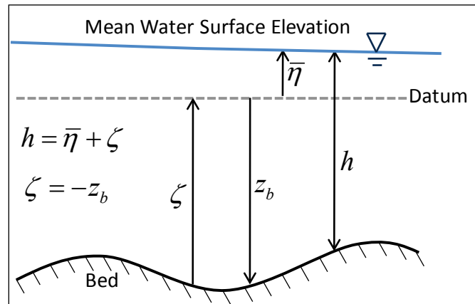
Figure 2-1. Vertical conventions used for the bed and mean water surface elevation.
